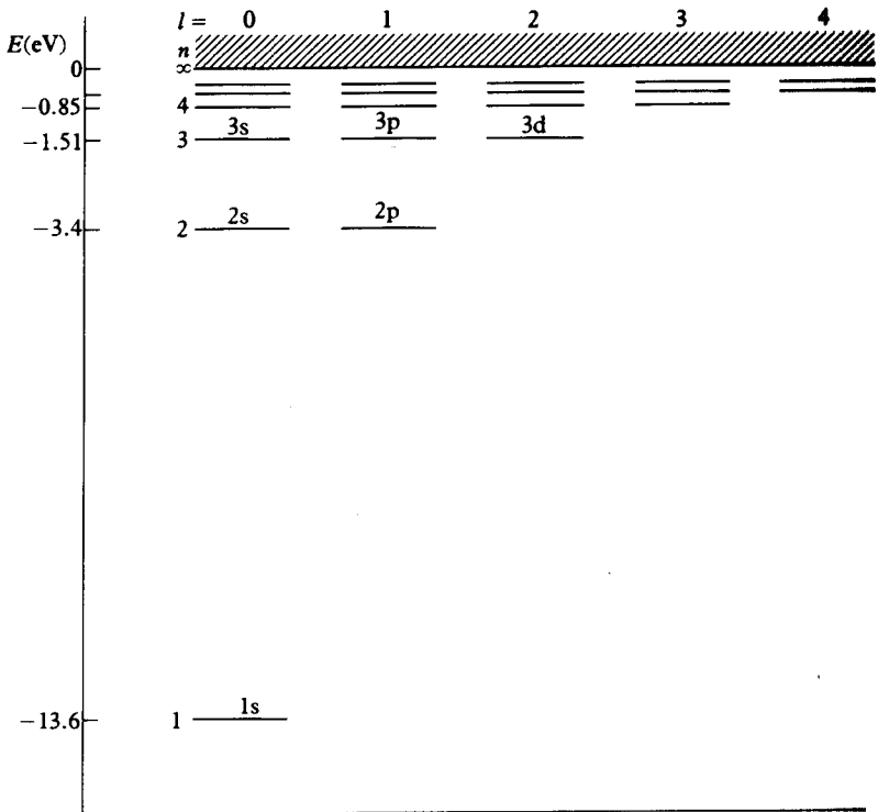
3.2 Energy-level diagram for atomic hydrogen.
